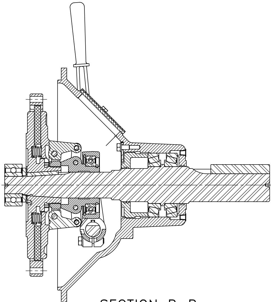
SECTION B-B
